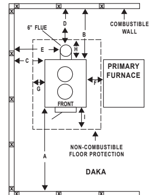
CLEARANCES TO COMBUSTIBLES FLOOR PROTECTION
