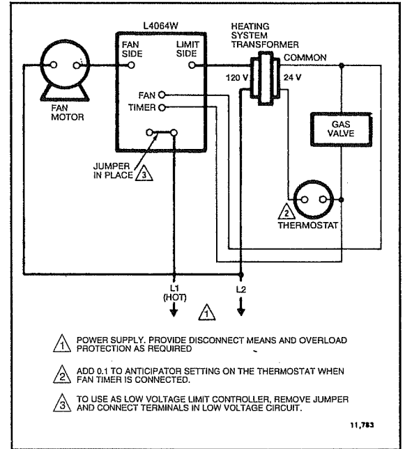
Fig. 6—L4064 3-wire line voltage hookup.
