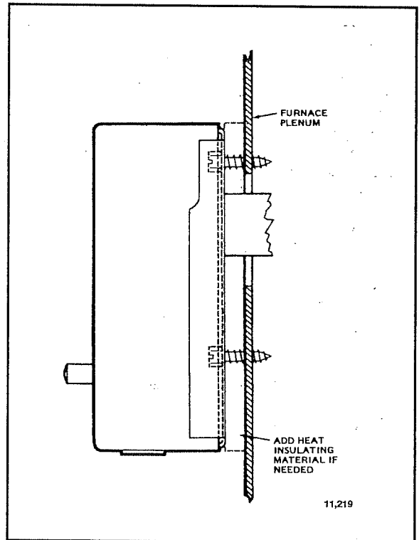
Fig. 1—Surface mounting requires a hole 13/16 in. [20.6 mm] diameter element insertion.
