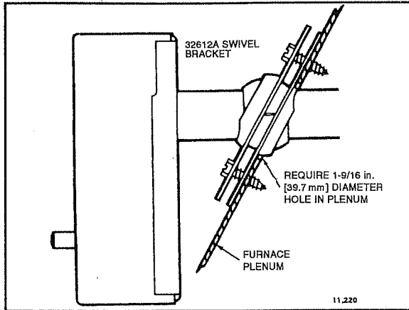
Fig. 2—Swivel mounting requires a 1-9/16 in. [39.7 mm] diameter mounting hole for element insertion.
