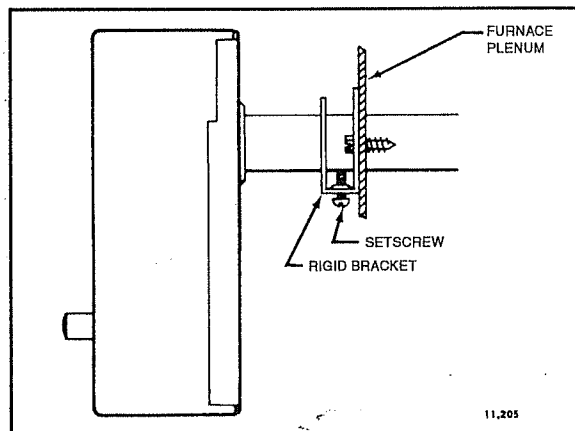
Fig. 3- Rigid bracket mounting requires a hole 13/16 in. [20.6 mm] diameter for element insertion.
